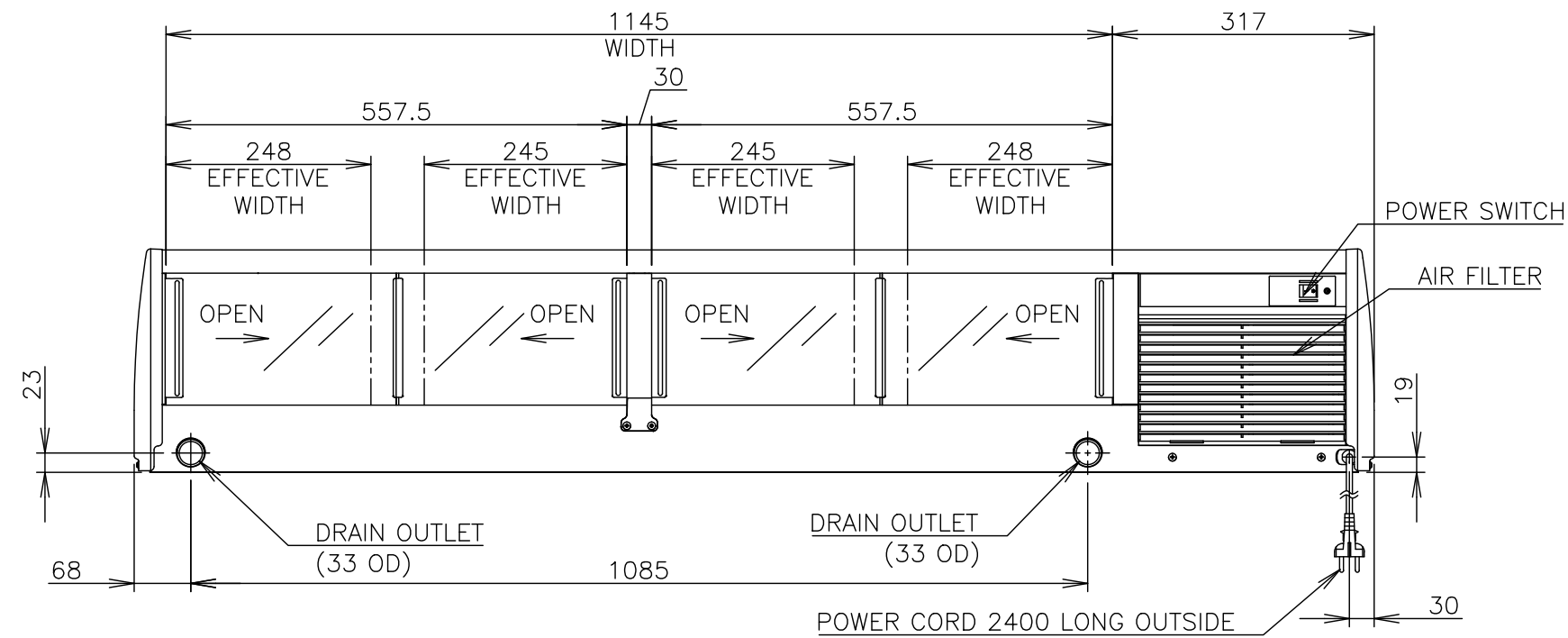
VIEW A(REAR)
