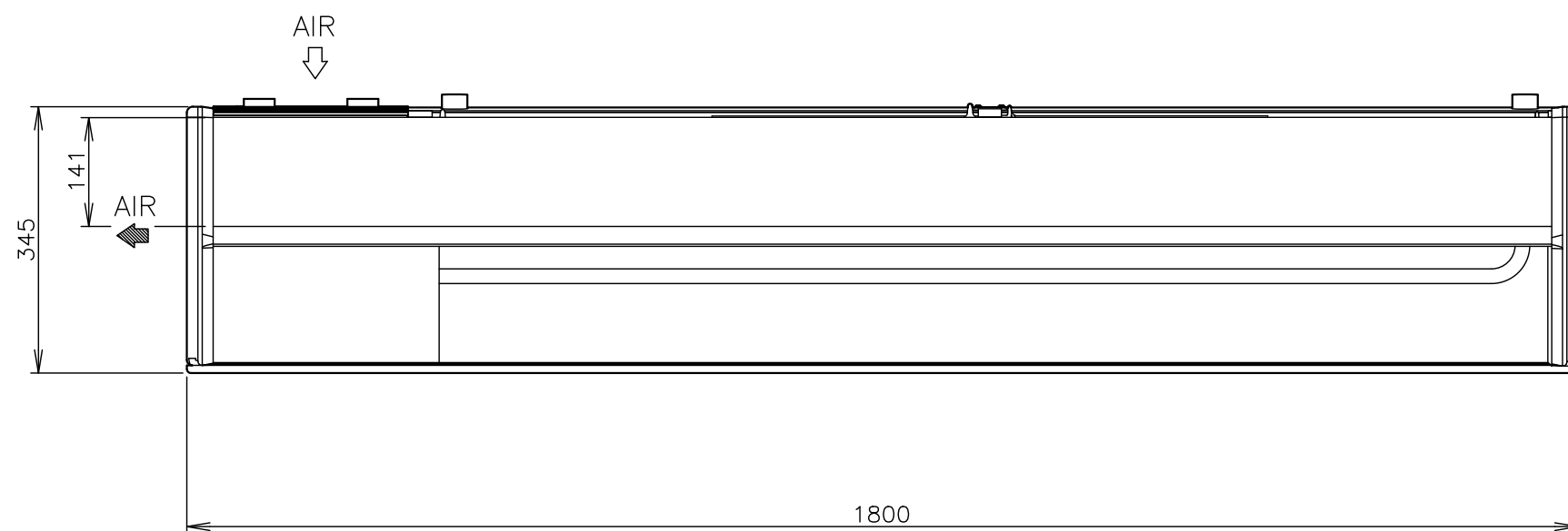
VIEW A(REAR)
