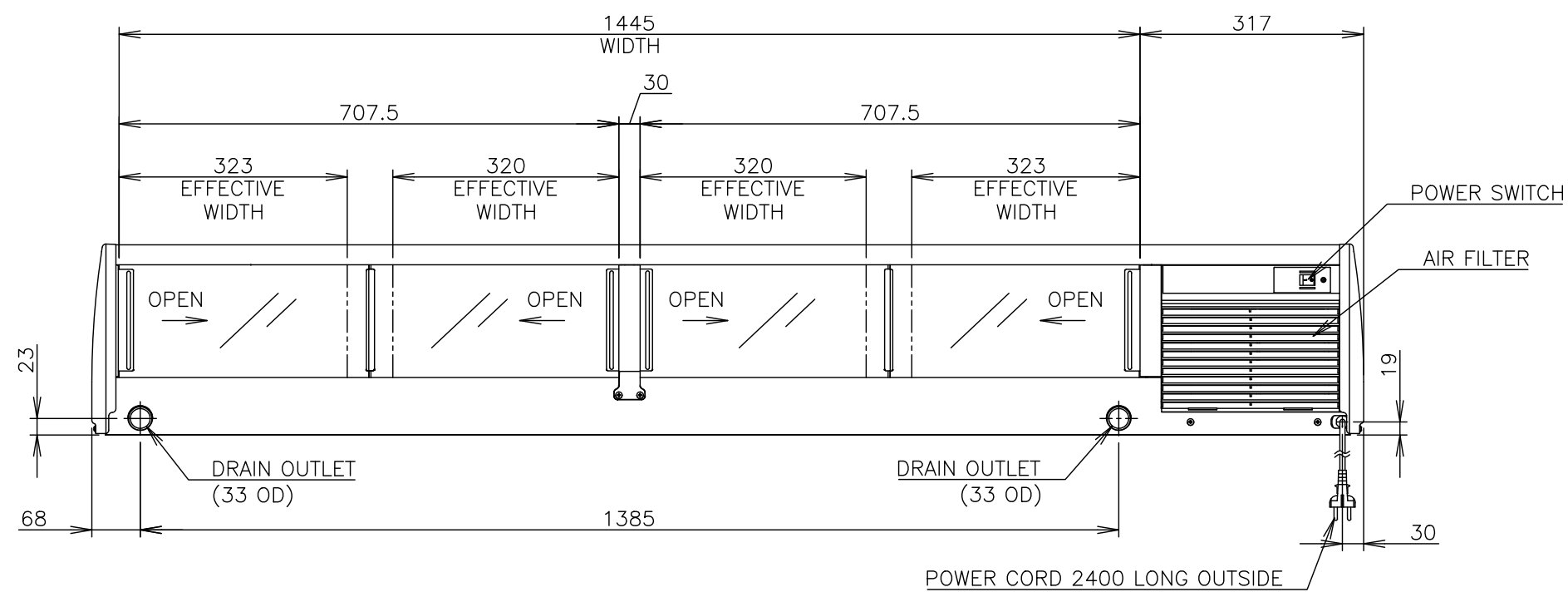
VIEW A(REAR)
