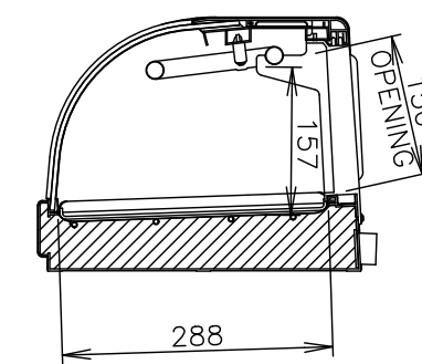
SECTIONAL SIDE VIEW
