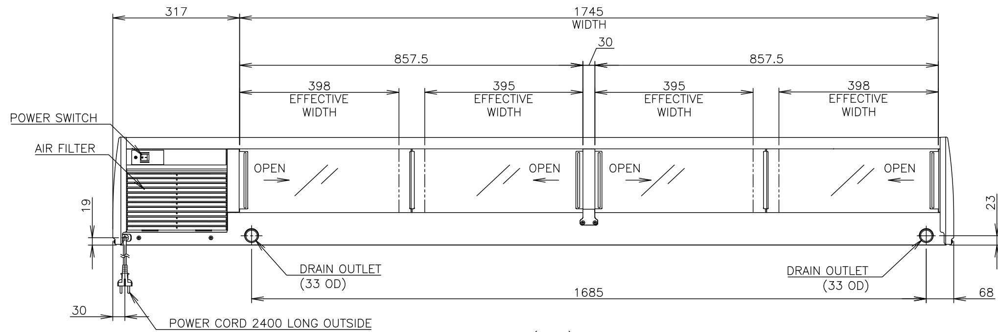
VIEW A(REAR)
