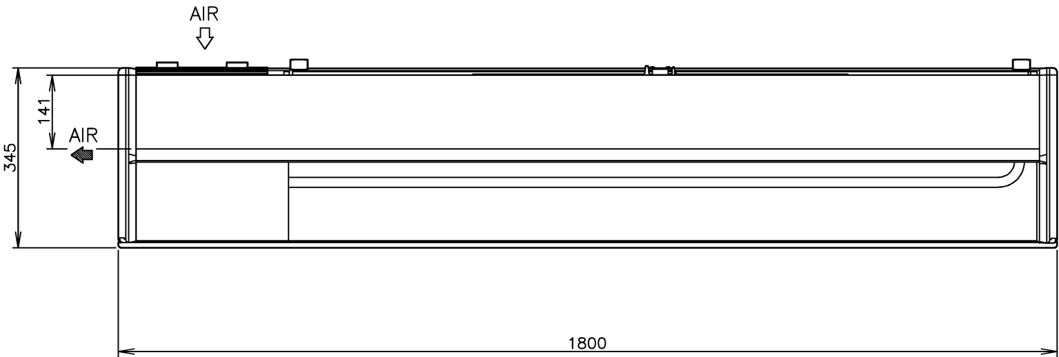
VIEW A(REAR)
