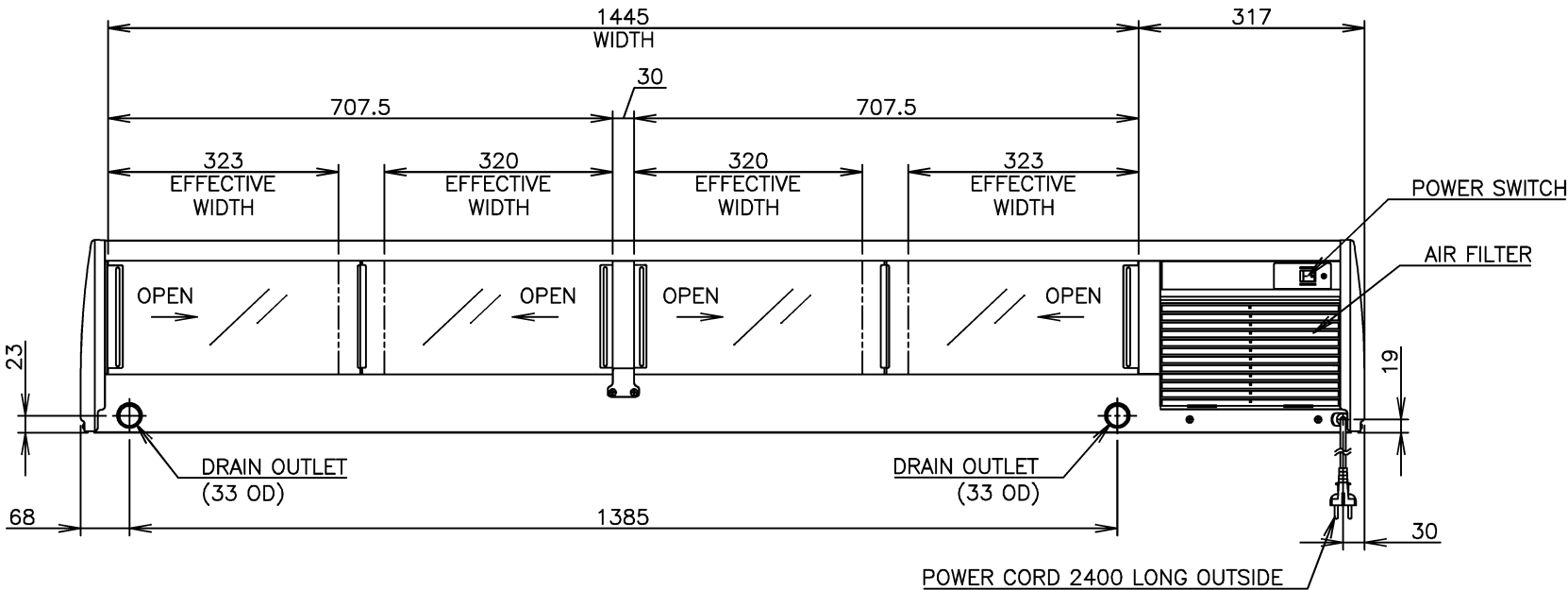
VIEW A(REAR)
