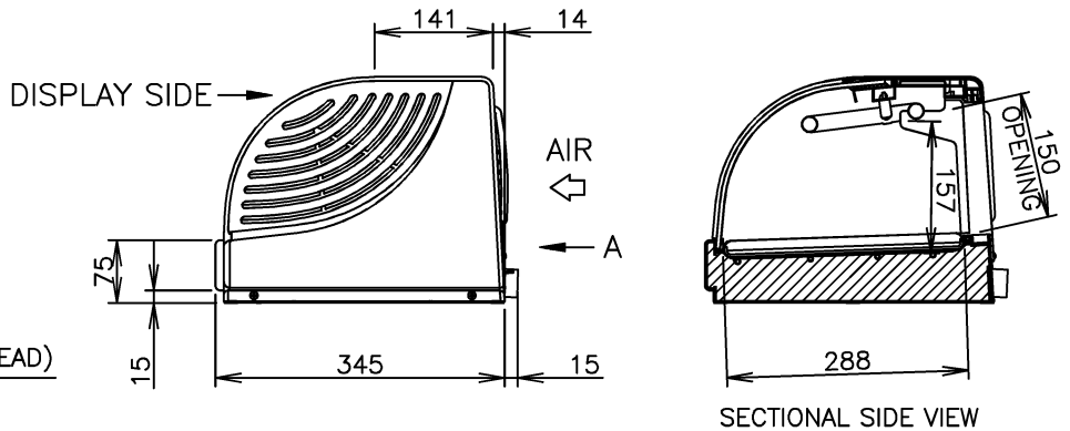
SECTIONAL SIDE VIEW
