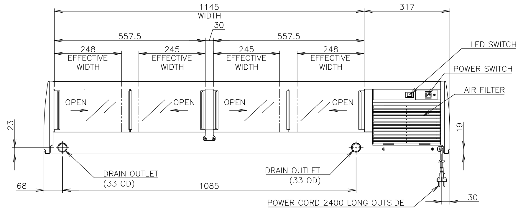
VIEW A(REAR)
