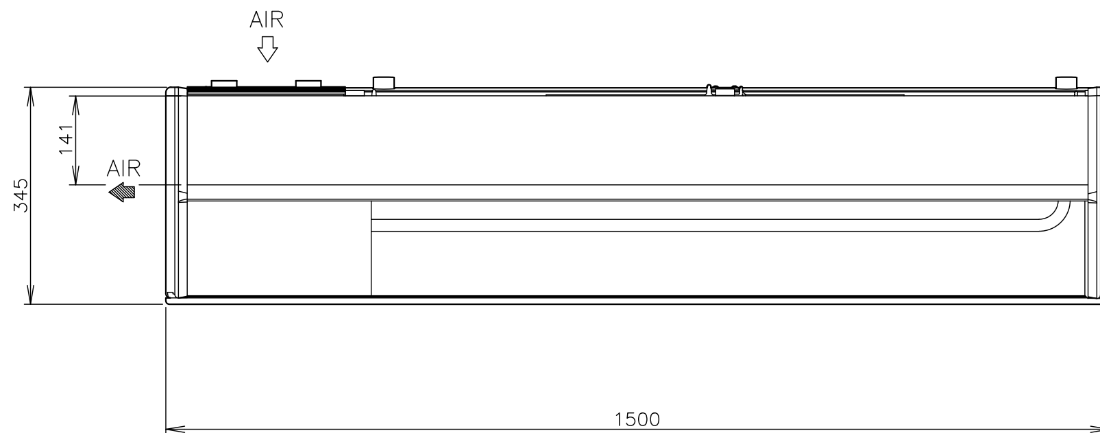
VIEW A(REAR)
