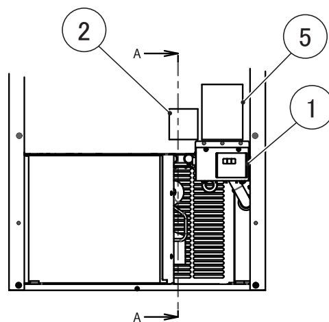
Front view with FRONT COVER LOWER ASSY removed
