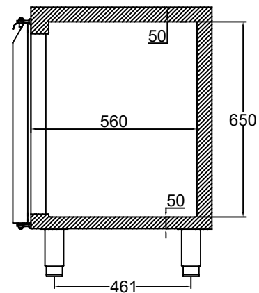
SECTION B-B
